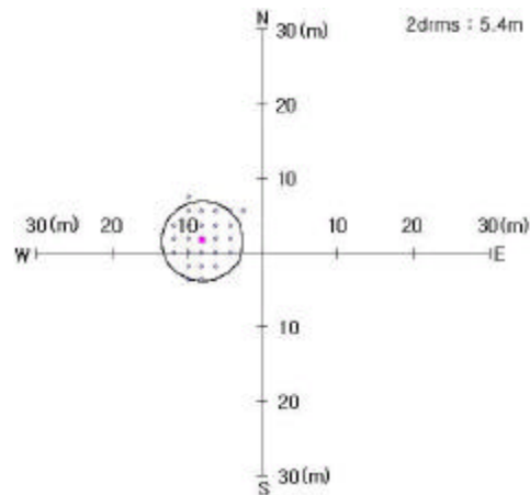
Fig. 3. The DGPS positioning accuracy for single reference station at Yosu harbor.
