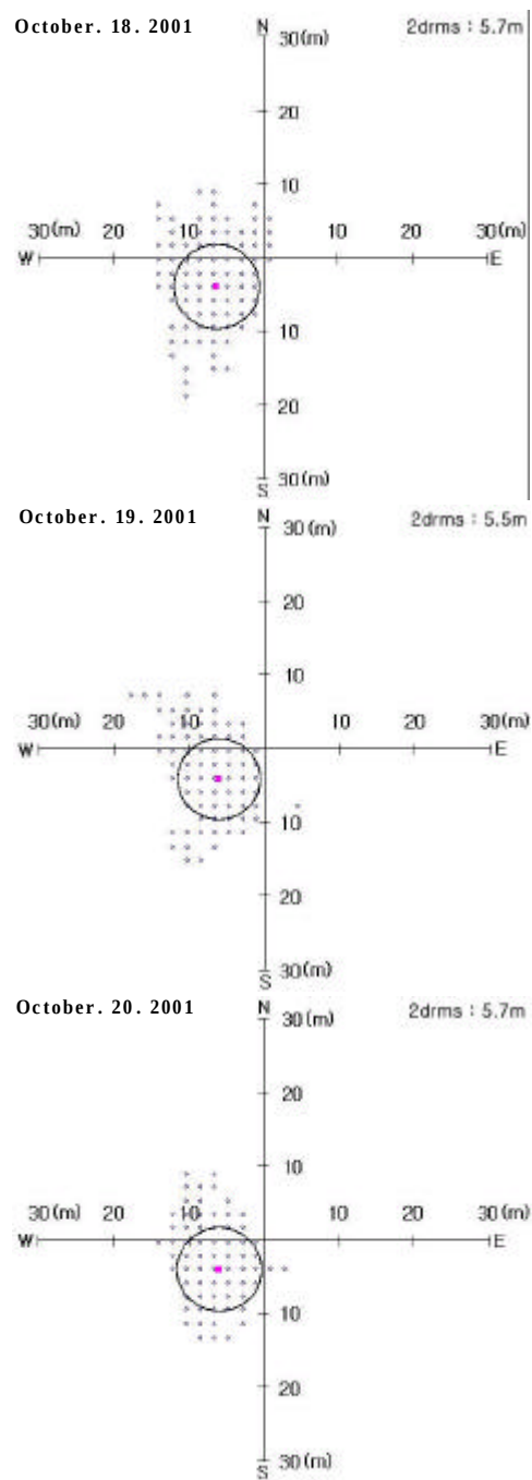
Fig. 4. The DGPS positioning accuracies for single reference station at Pukyong national university.
