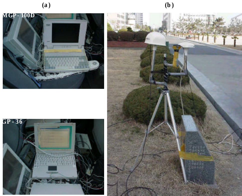
Fig. 1. Configuration for the DGPS system.
