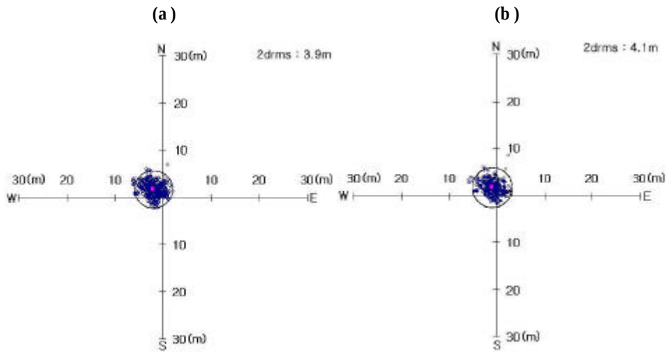
Fig. 5. The DGPS positioning Accuracies for multiple reference station at Yosu harbor.
