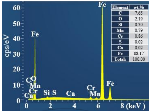
Fig. 6. Spectrum of fracture surface components.
