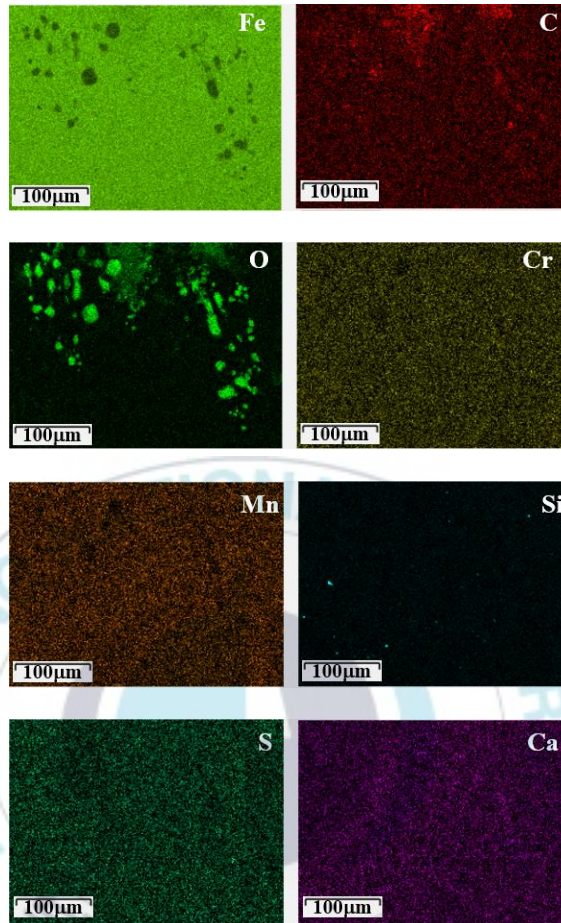
Fig. 5 EDS layered image of fracture surface components.
