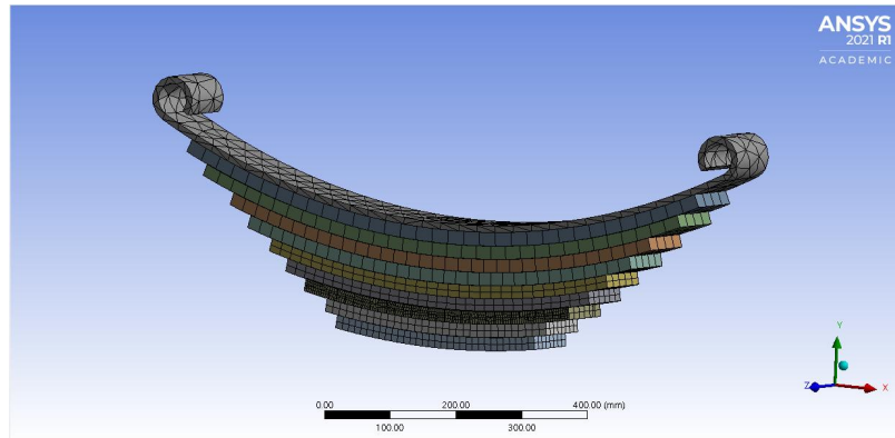
Fig. 8 FE analysis modeling for leaf spring.
