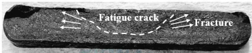
Fig. 3 Observation of the macro fracture surface of a leaf spring.
